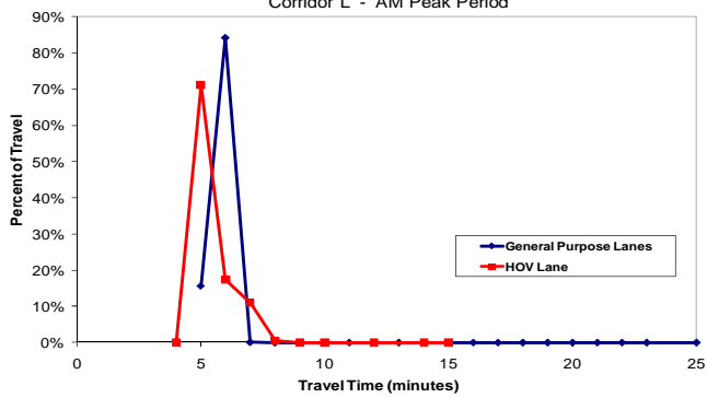
Travel Time Distribution US60 Westbound: Loop 202 Redtan TI to Val Vista Drive, 6.12 miles Corridor L - AM Peak Period
