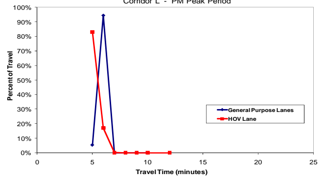
Travel Time Distribution US60 Eastbound: Val Vista Drive to Loop 202 Redtan TI, 6.12 miles Corridor L - PM Peak Period
