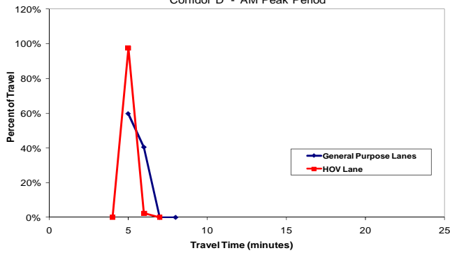
Travel Time Distribution I-10 Maricopa Eastbound: US60 to Chandler Boulevard, 5.76 miles Corridor D - AM Peak Period
