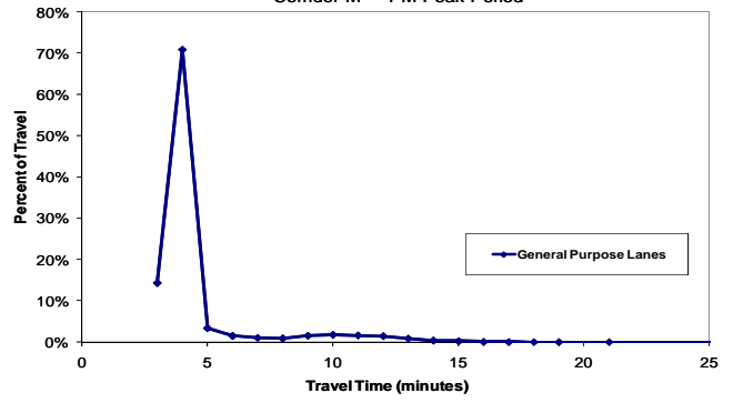
Travel Time Distribution SR143 Southbound: I-10 Maricopa Freeway to Loop 202, 3.58 miles Corridor M - PM Peak Period
