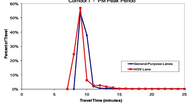
Travel Time Distribution Loop 202 Westbound: Loop 101 to I-10/SR51, 9.47 miles Corridor I - PM Peak Period
