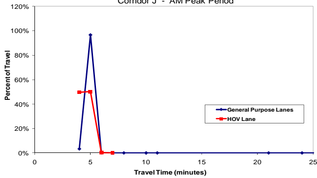
Travel Time Distribution US60 Eastbound: I-10 to Loop 101, 4.45 miles Corridor J - AM Peak Period
