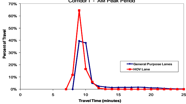
Travel Time Distribution Loop 202 Westbound: Loop 101 to I-10/SR51, 9.47 miles Corridor I - AM Peak Period
