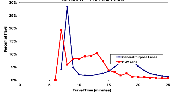
Travel Time Distribution I-10 Maricopa Eastbound: SR51 to US60, 8.03 miles Corridor C - PM Peak Period
