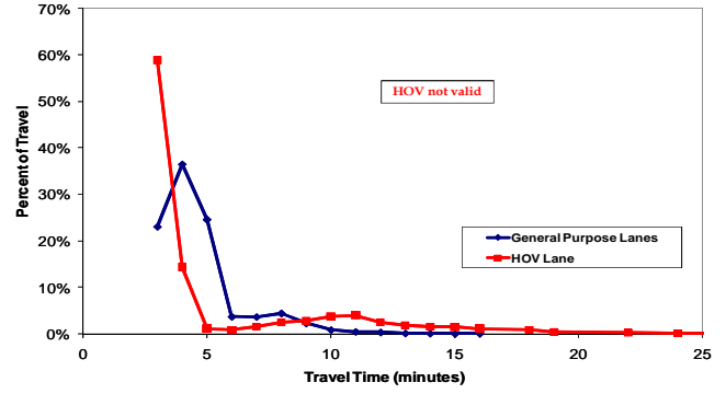
Travel Time Distribution Loop 101 Southbound: Loop 202 Red Mountain to US60, 3.33 miles Corridor O - PM Peak Period
