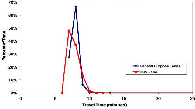
Travel Time Distribution I-10 Papago Westbound: I-17 to 83rd Avenue, 7.83 miles Corridor A - AM Peak Period
