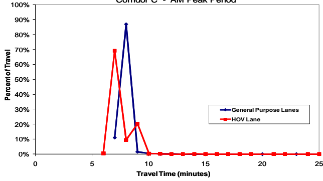
Travel Time Distribution I-10 Maricopa Eastbound: SR 51 to US 60, 8.03 miles Corridor C - AM Peak Period
