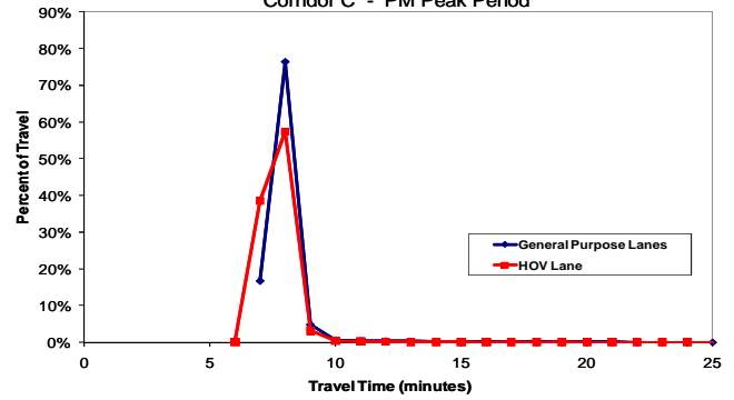
Travel Time Distribution I-10 Maricopa Westbound: US60 to SR51, 8.03 miles Corridor C - PM Peak Period
