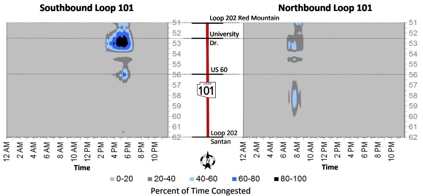
Figures 2.XX Percent of Time Congested on Loop 101 (2009)
