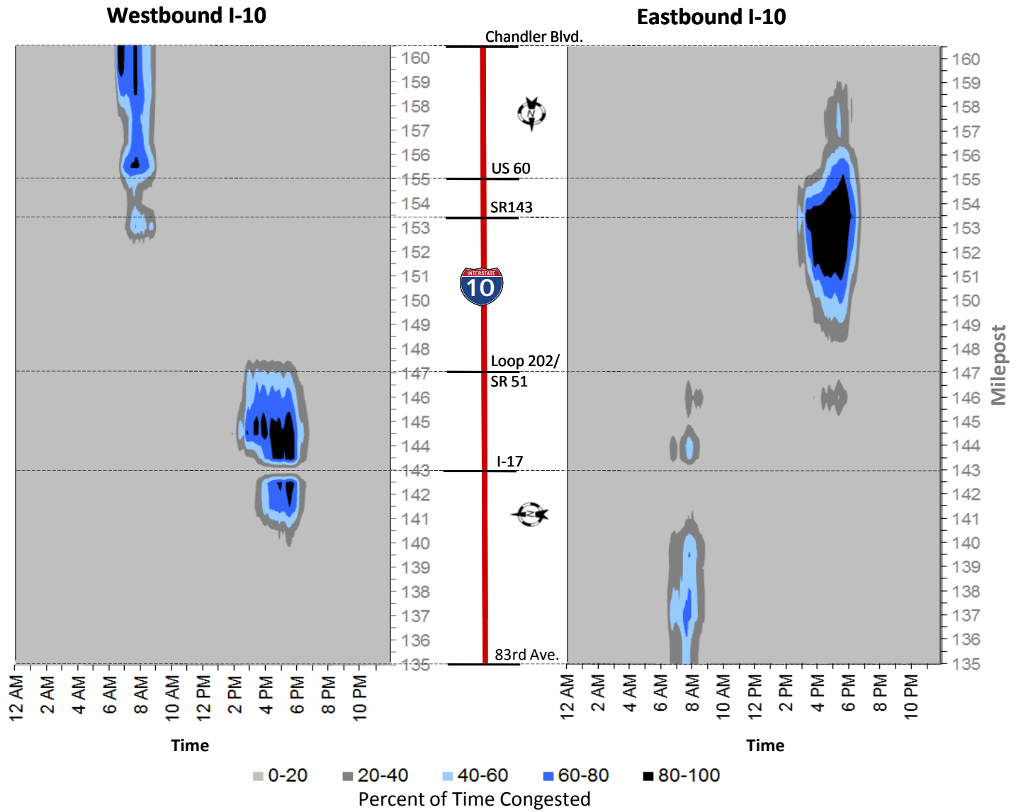
Figure 2.XX Percent of Time Congested on I-10 (2009)
