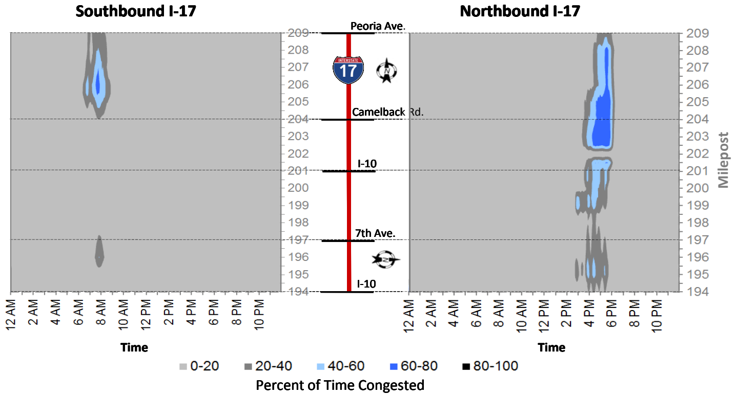
Figures 2.XX and 2.XX Percent of Time Congested on I-17 (2009)
