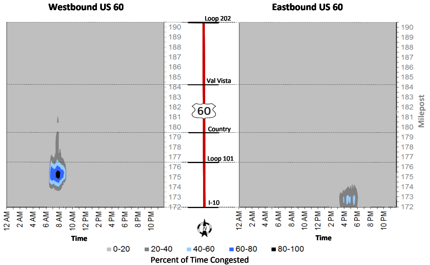
Figures 2.XX and 2.XX Percent of Time Congested on US 60 (2009)
