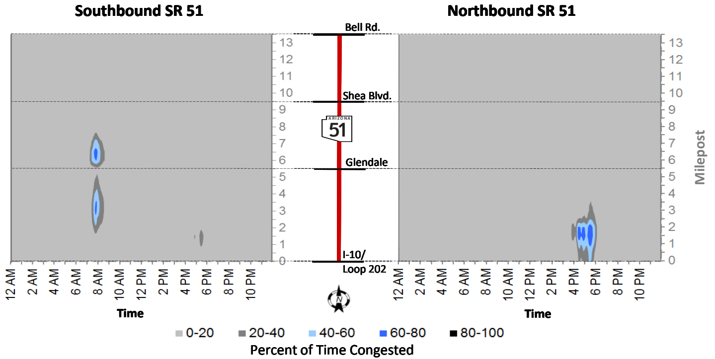
Figures 2.XX and 2.XX Percent of Time Congested on SR 51 (2009)
